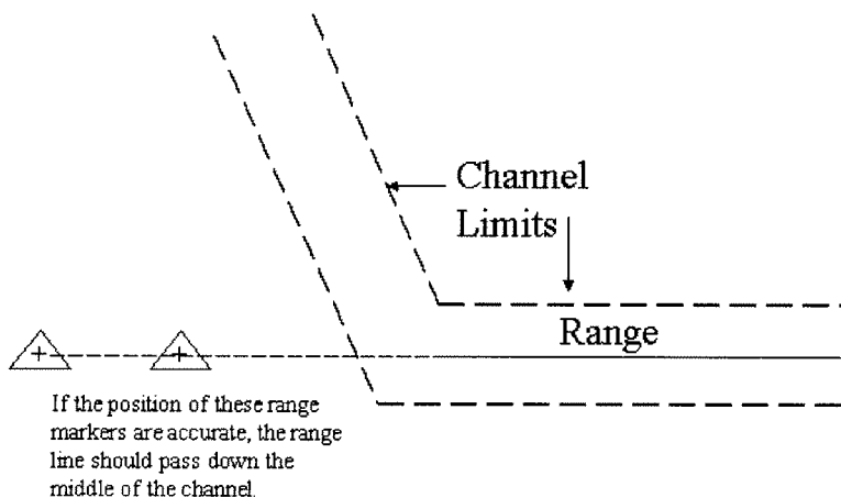
Figure 1 - Navigational Range aligning with channel
